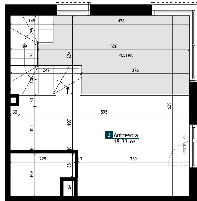
ANTRESOLA
