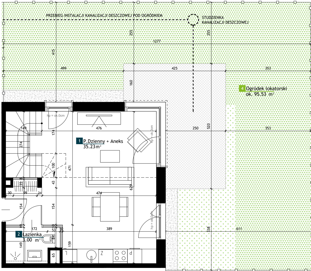
PARTER
